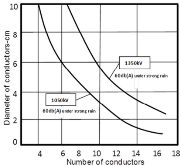
Figure 5-21: Diameter and number of conductors in the bundle to limit noise level to 55-60 dB, at 15 m from the outer phase during wet conditions
