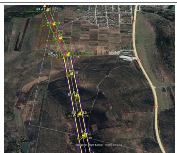
Fig. 5-5: The 400 kV OHTL passes on the territory of the com. Bacioi (Straisteni)
