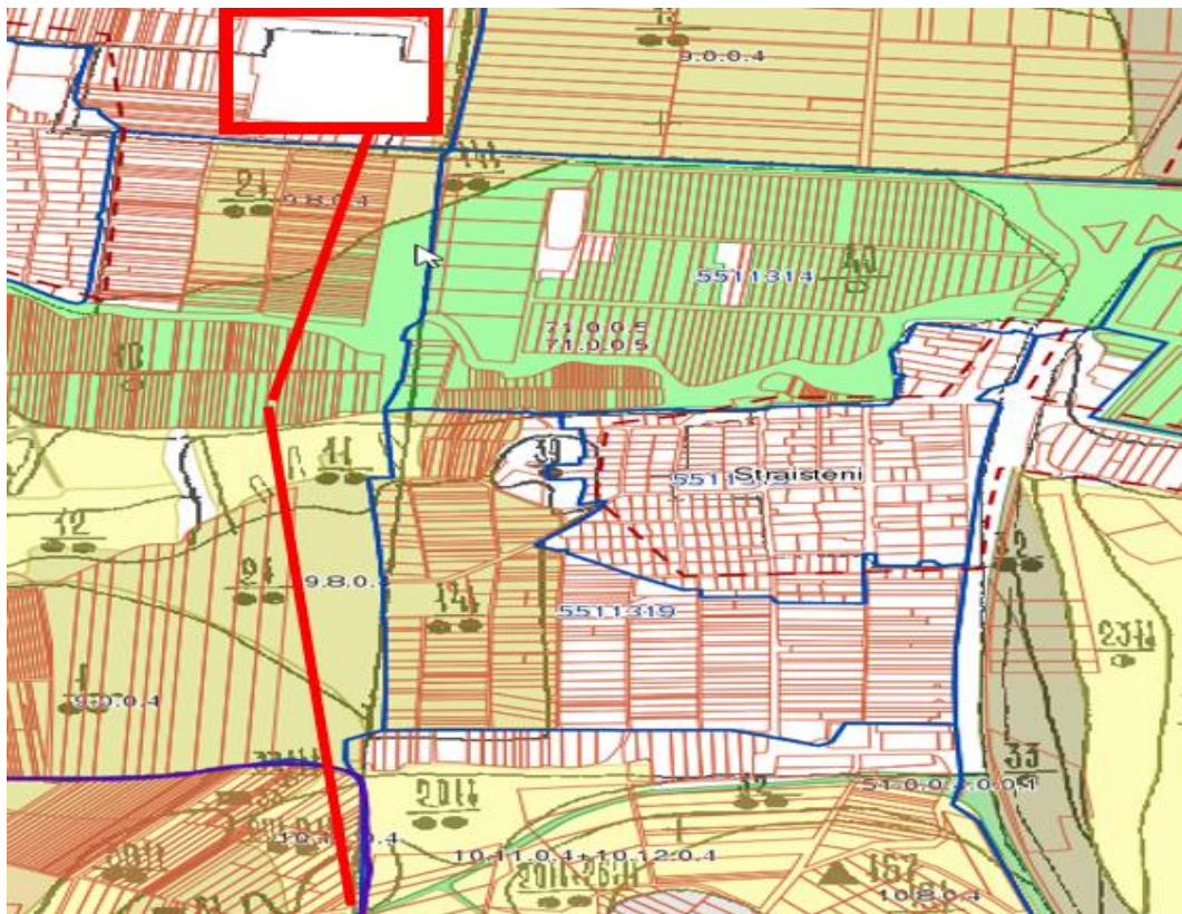
Figure 5-14: Soils types 54 within the commune Bacioi
