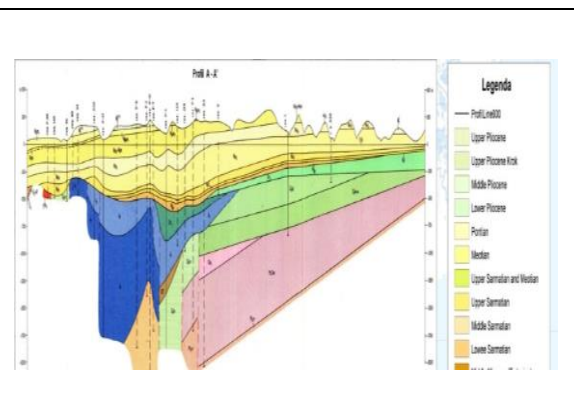
Fig. 5-13: The profil A-A of the geological structure
