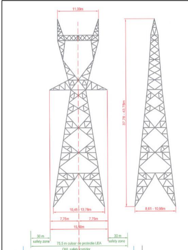
Fig. 3-9: The 400 kV OHTL tension tower type "Y" (longitudinal view/ lateral view)
