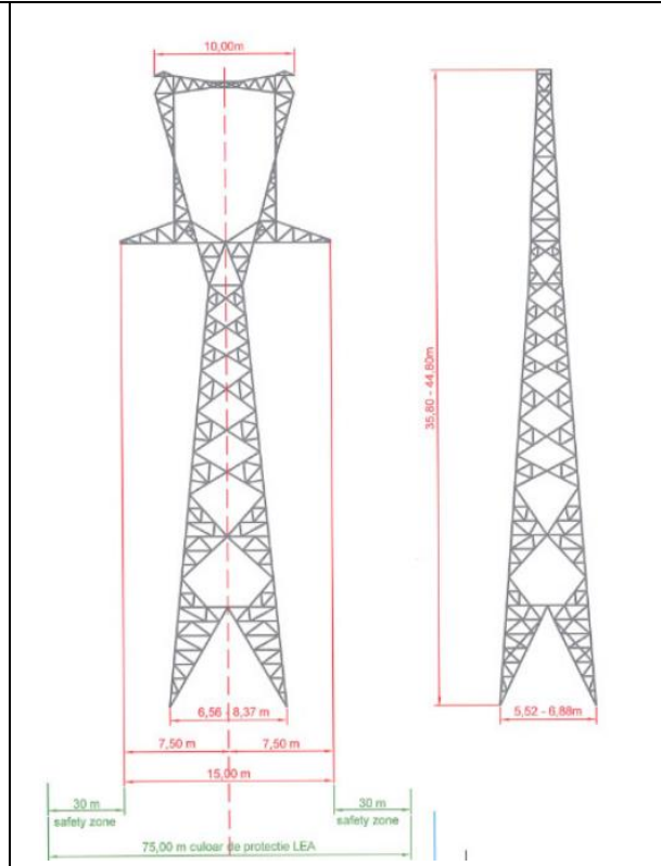
Fig. 3-10: The 400 kV OHTL suspension tower type "Y" (longitudinal view/ lateral view)
