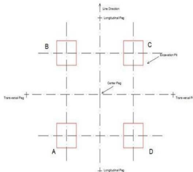
Figure 3-11 The tower foundation
