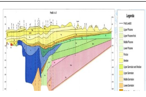
Fig. 5-14: The profil A-A of the geological structure
